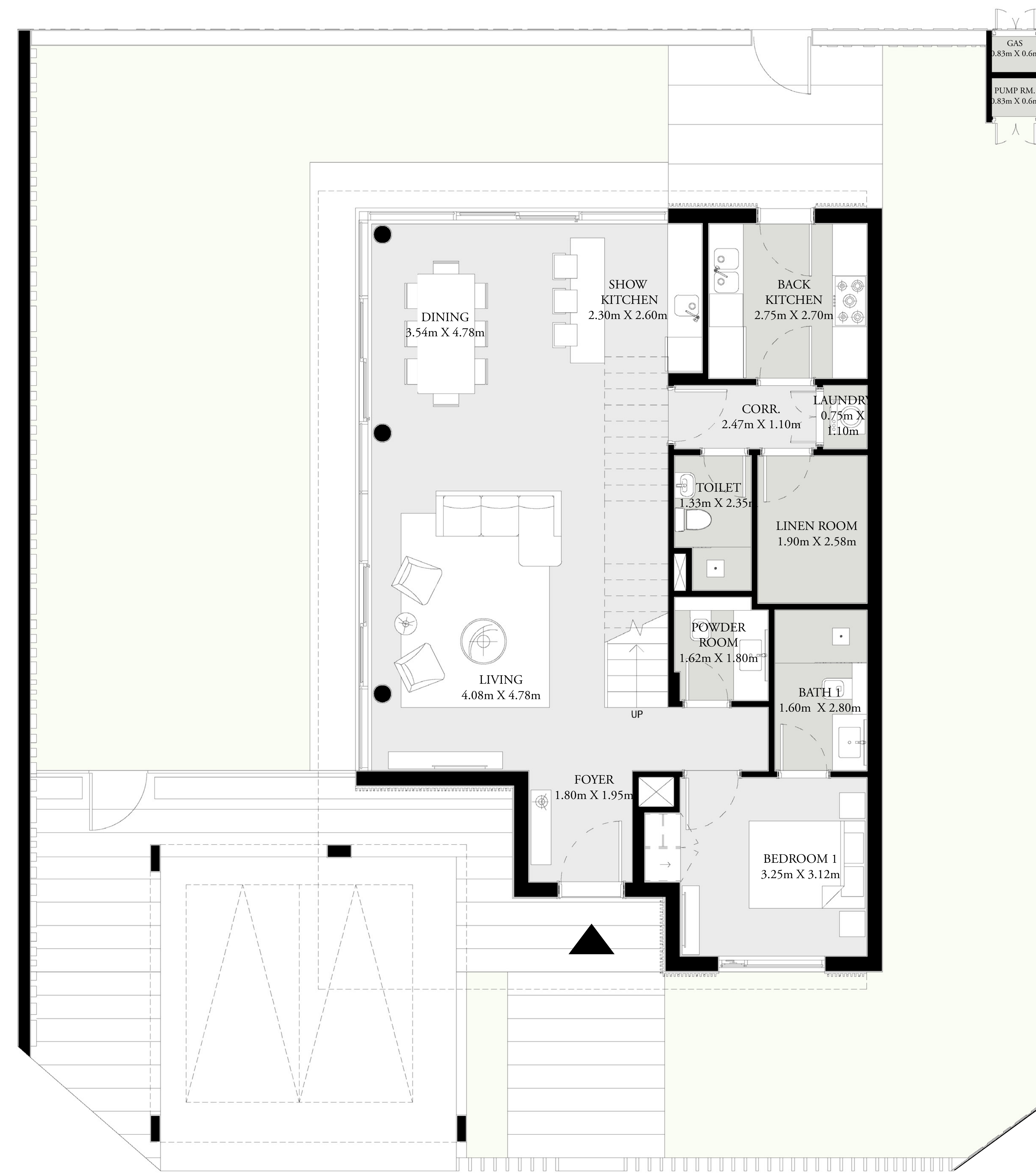
GROUND FLOOR
