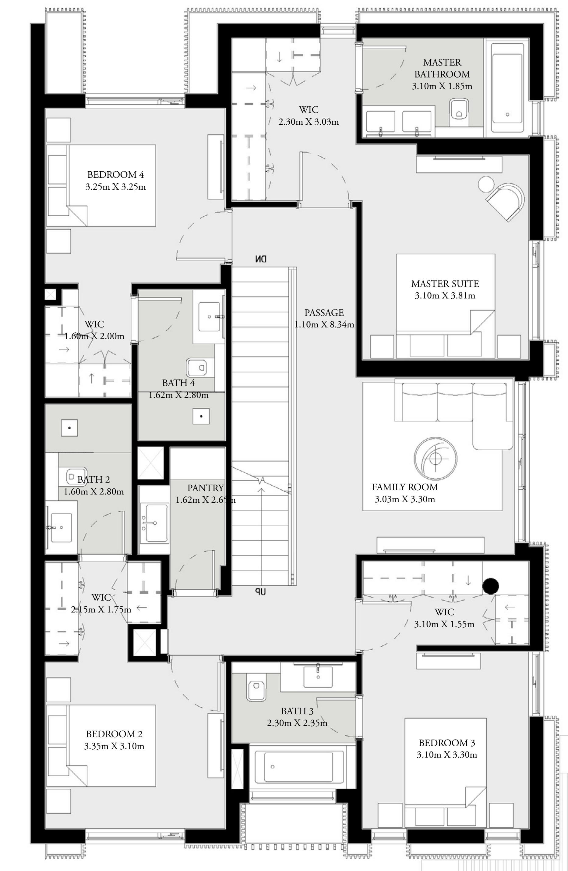
FIRST FLOOR
